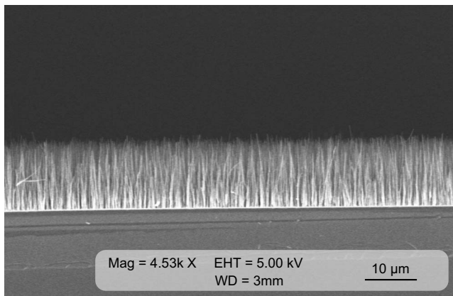
FIG. 2. SEM image showing cross section of aligned carbon nanofibers grown on a silicon substrate.
