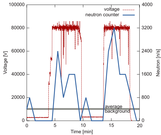
FIG. 4. (Color online) Neutron yields (at the target) from the CNF sample at a deuterium gas pressure of 0.08 Pa and a gas cracker power of 60 W.
