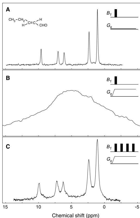
Fig. 2. (A) One-pulse proton spectrum of trans-2-pentenal (eight scans). The linewidth ( \sim 40 Hz) is dominated by the intrinsic residual inhomogeneity of the magnetic field. (B) Spectrum of trans-2-pentenal (64 scans, 2.2 kHz full width at half maximum line broadening) in the presence of a linear static field gradient of 0.12 mT/cm ( \sim 5 kHz/cm) along the sample axis. An exponential apodization of 50 Hz was applied to enhance the signal to noise ratio. (C) Proton spectrum obtained with the refocusing sequence of Fig. 3B after 64 scans, in the presence of the same field gradient. Constant-rotation composite \pi/2 pulses were implemented by the series (2\gamma)_{97.2}(4\gamma)_{291.5}(2\gamma)_{97.2}(\gamma)_0 , where \gamma represents a nominal \pi/2 pulse (13). The total duration was 117 \mu\text{s} ; \tau_\beta , the length of the \beta pulse, was 23 \mu\text{s} for an evolution time \tau_{\text{dw}} set at 250 \mu\text{s} . After processing the FID, the frequency units were shifted so that the position of the most intense peak matched the corresponding peak observed in (A). Even though the linewidth is slightly increased, all nonequivalent proton resonances are resolved and the full chemical shift information is recovered.
