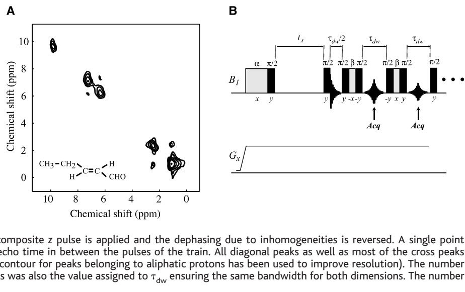
Fig. 4. (A) Two-dimensional correlation spectrum (absolute value mode) of trans-2-pentenal obtained through (B) an adapted COSY sequence under conditions identical to those of Fig. 2B. A linear static field gradient of 0.12 mT/cm (~5 kHz/cm) along the sample axis spreads the Larmor frequencies in both dimensions over a range of 20 ppm, and no relevant spectroscopic information can be recorded with a standard experiment. In the present case, however, the evolution period is made insensitive to field inhomogeneities by the use of a pulse [\alpha(\vec{r})]_x before the standard (\pi/2)_y excitation pulse. The duration of [\alpha(\vec{r})]_x is sequentially incremented in a manner proportional to t_1 . The ratio is adjusted so that the next (\pi/2)_y mixing pulse occurs synchronously with the nutation echo. In the direct dimension, the detection is made stroboscopically in a way similar to that of Fig. 2C. After a time \tau_{dw}/2 , a composite z pulse is applied and the dephasing due to inhomogeneities is reversed. A single point acquisition takes place at the expected nutation echo time in between the pulses of the train. All diagonal peaks as well as most of the cross peaks for J -coupled protons are regained (a higher level contour for peaks belonging to aliphatic protons has been used to improve resolution). The number of increments for t_1 was 64 in steps of 250 \mu s. This was also the value assigned to \tau_{dw} ensuring the same bandwidth for both dimensions. The number of scans for each evolution time t_1 was 8.
