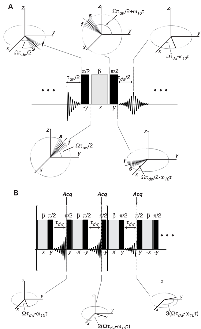
Fig. 3. (A) Rotating-frame classical diagram describing spin evolution under a train of z-rotation composite pulses. For the sake of clarity, the diagram only depicts nuclear spins with the same chemical shift but spread over different positions along the sample. During a free evolution period, equivalent spins dephase because of the spatial dependence of the Larmor frequency. "Faster" ("slower") spins, located closer to (away from) the excitation coil, have been labeled by a small f ( s ) in the diagram. A position-dependent phase correction is possible through the pulse series (\pi/2)_{-y}[\beta(\vec{r})]_x(\pi/2)_y . (Perfect) constant-rotation composite \pi/2 pulses tip the spins back and forth between the xy and yz planes. In the region of the sample where the static and rf field gradients are matched, a [\beta(\vec{r})]_x pulse applied over the proper time period gives rise to an overall phase shift that exactly reverses the relative positions of (chemically equivalent) fast and slow spins and induces a subsequent nutation echo. Because the same phase shift equally affects nuclei with different chemical shifts, the echo amplitude fully preserves the accumulated phase differences between chemically inequivalent spins. (B) Pulse train actually used during the experiment. An initial dephasing induced by the pulse [\beta(\vec{r})]_x is refocused during the free evolution (or dwell time) period. A one-point acquisition takes place at the nutation echo maximum, just before the next (\pi/2) pulse. At each step in the train, a phase alternation is performed to compensate for undesired evolution during the rf irradiation. The entire rf sequence—indicated by surrounding brackets in the drawing—is repeated, with stroboscopic detection providing the inhomogeneity-free free induction decay. The constant phase shift \omega_{10}\tau_\beta remaining at each step of the train can be corrected by sequentially adjusting the phase of the rf pulses or by a shift of the reference frequency in the measured spectrum after data processing.
