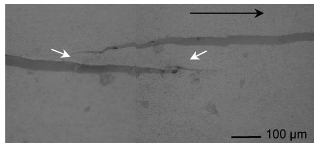
Fig. 8. Optical micrograph showing crack bridging by uncracked ligaments (indicated by white arrows) in dentin dehydrated using methanol. The black arrow indicates the nominal direction of crack growth.
