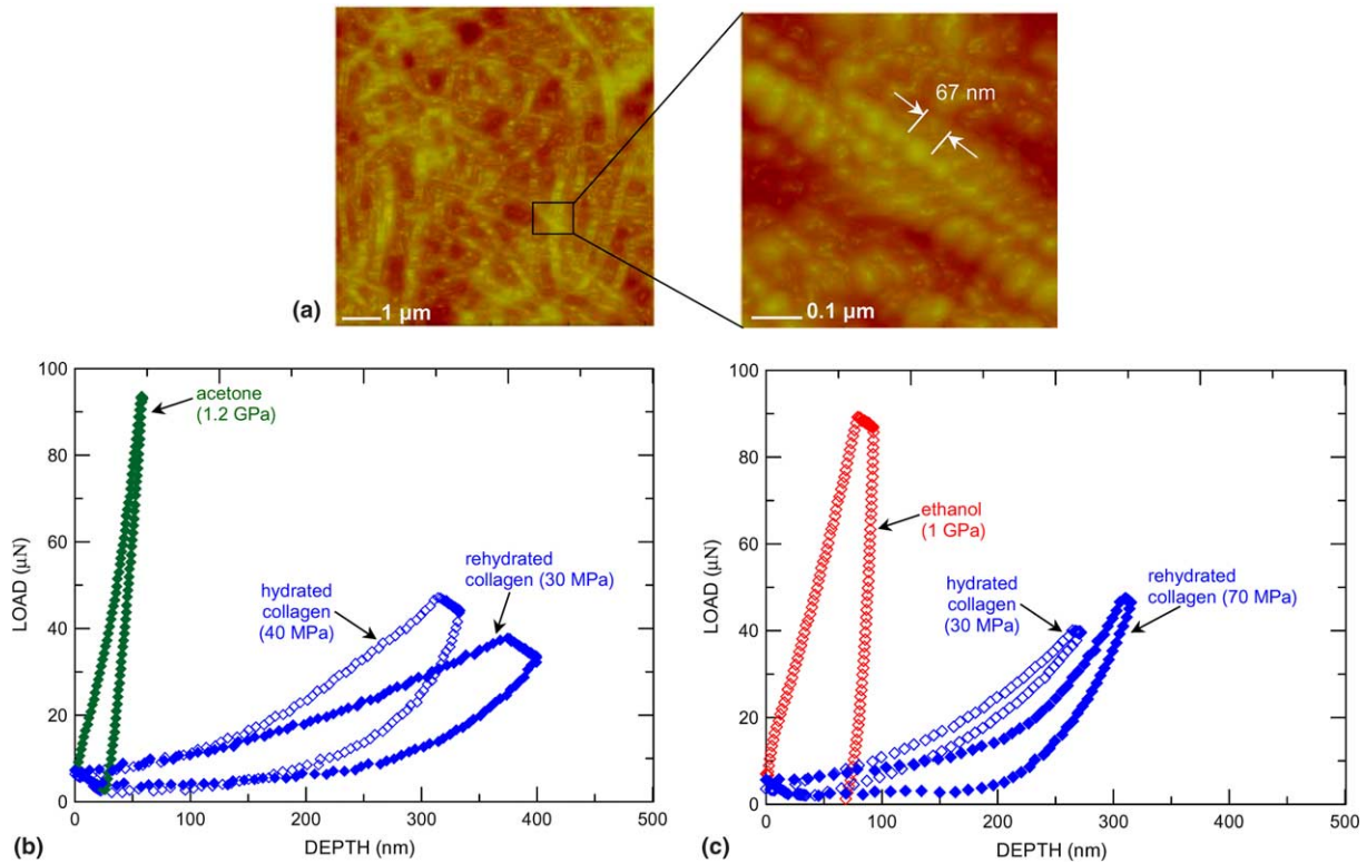
Fig. 5. (a) AFM images of hydrated collagen fibers. Note the regular “banded” structure as indicated in the higher magnification micrograph (right). Typical load–displacement data obtained for AFM-based “hydrated/dehydrated/rehydrated” nanoindentation of individual collagen fibers for the (b) water/acetone/water, and (c) water/ethanol/water cases are shown (numbers in brackets are calculated reduced elastic moduli). Note the dramatic increase in the modulus (slope of initial portion of the unloading curve) upon chemical dehydration.
