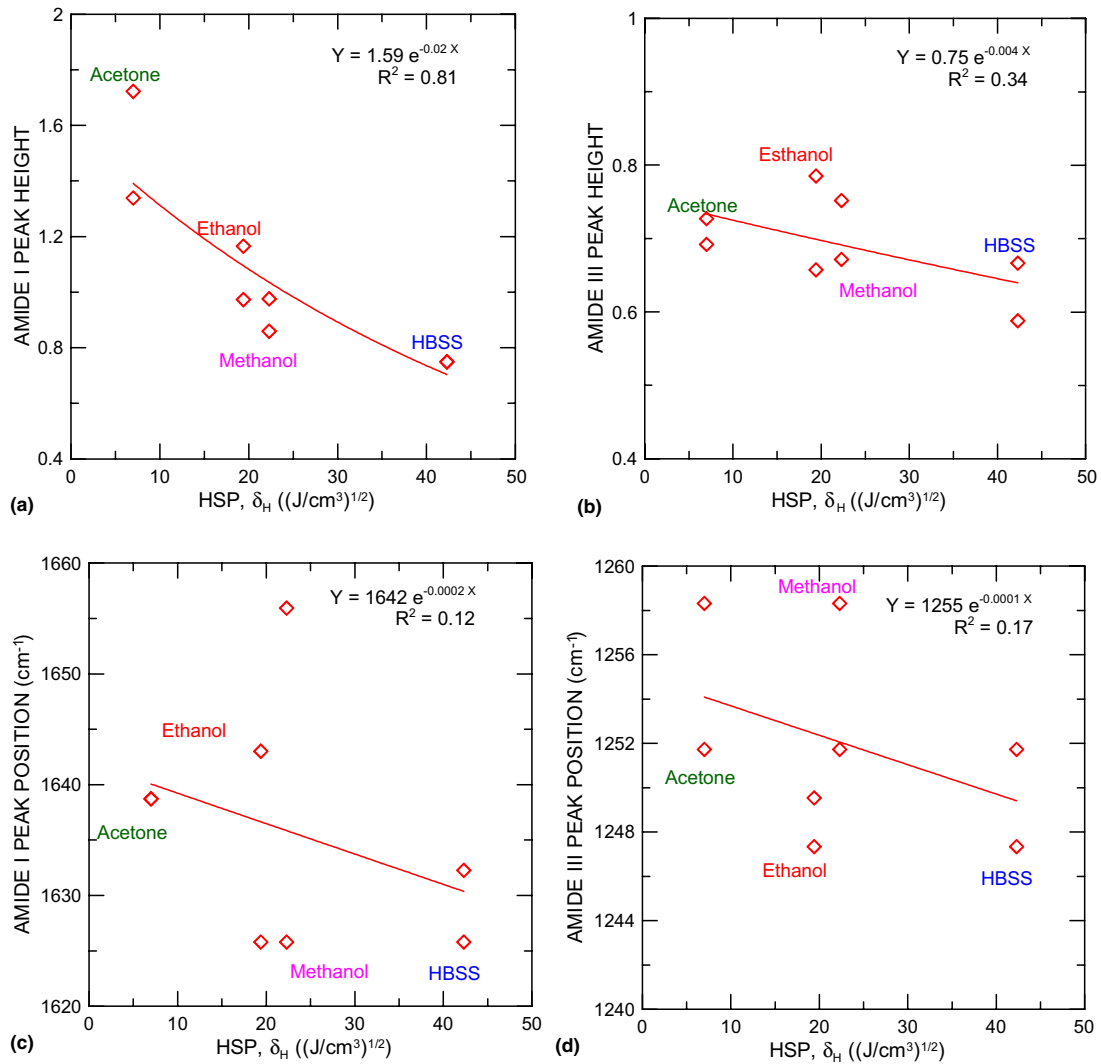
Fig. 7. Variation of the amide I and amide III peak positions and peak heights (normalized to the height of the \text{CH}_2 wag peak) with Hansen Solubility Parameter (HSP) for hydrogen bonding forces, \delta_H . The exponential fit for the data and the corresponding coefficient of determination, R^2 , are given at the top right corner of each plot.
