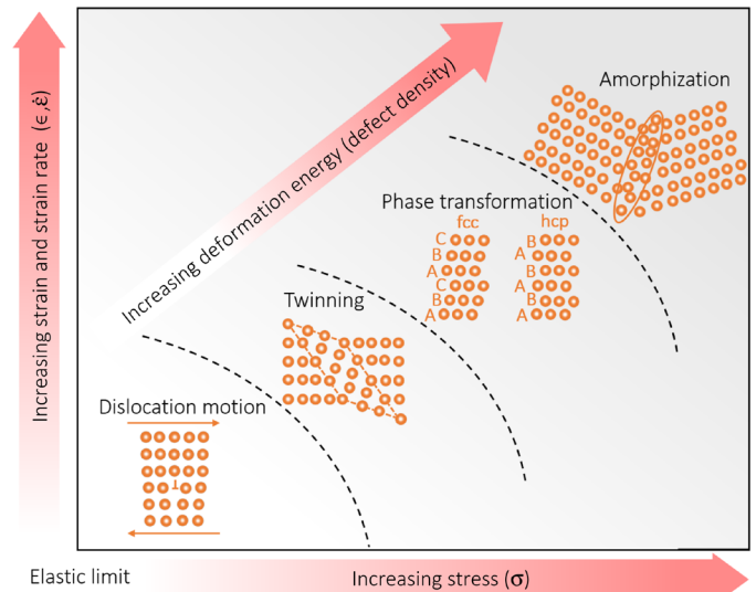
Fig. 4. Proposed hierarchical deformation mechanism paradigm for the equiatomic CrCoNi-based HEAs subjected to increasing degrees of deformation. Elastic deformation, dislocation-mediated plasticity, twinning-induced plasticity, TRIP, and finally solid-state amorphization. Triggering the next mechanism requires the generation of additional defects, i.e., dislocations and/or point defects (vacancies). These multiple mechanisms can interact, leading to a synergy of strengthening processes and a resulting highly complex microstructure.
