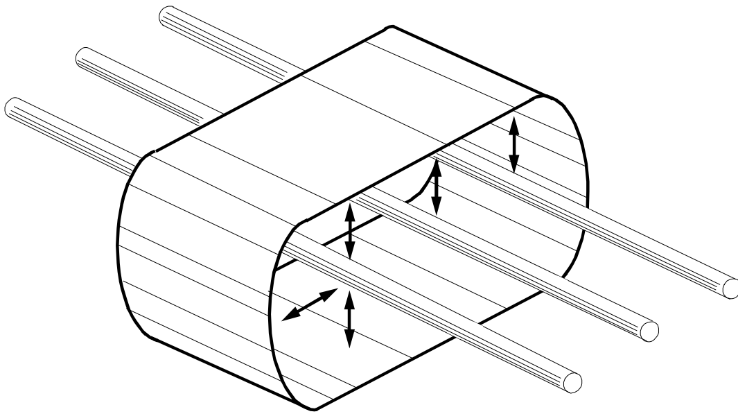
Figure 15-15. Danger zone for cranes and lifted loads operating near electrical transmission line. (See Table 15-3 for minimum radial distance of prohibited zone.)
