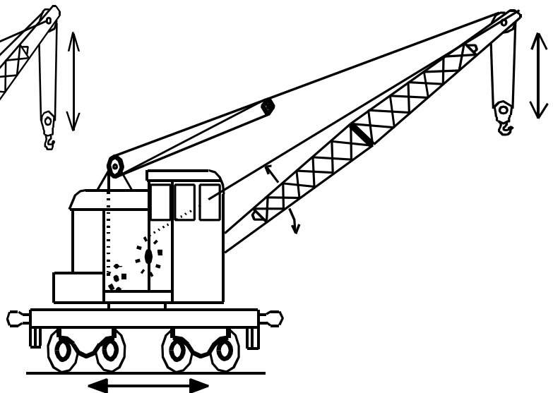
Figure 15-4. Locomotive crane.
