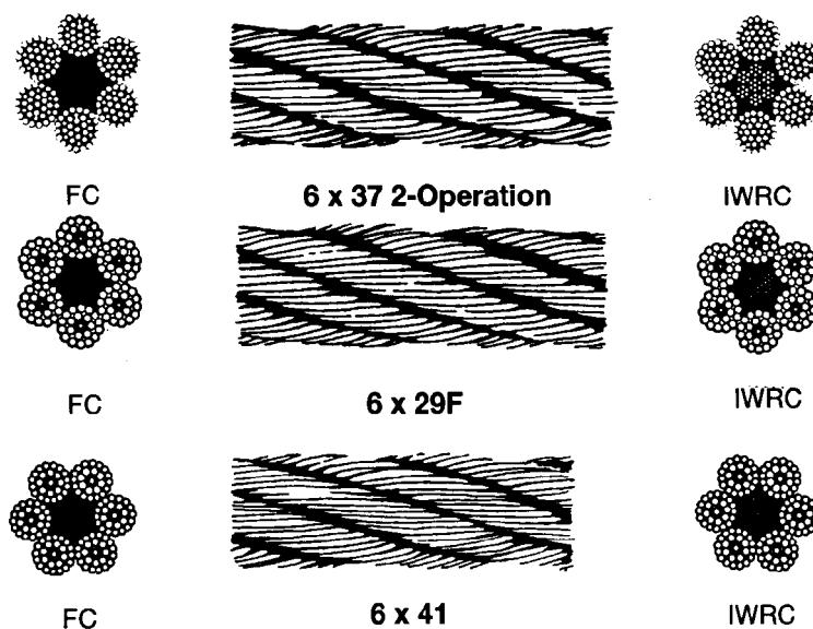
Figure 11-5. 6 x 37 classification of wire rope.
