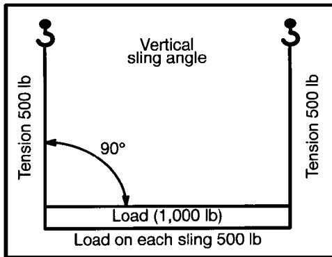
Figure 11-6. Balancing loads.
