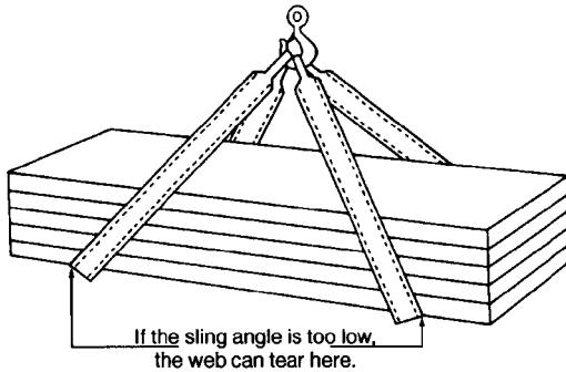
Figure 11-20. Effect of low sling angle.
