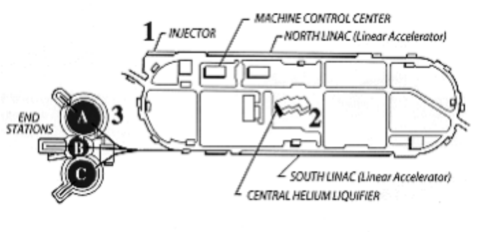
Fig. 11-5. The electron accelerator at Thomas Jefferson Laboratory.
