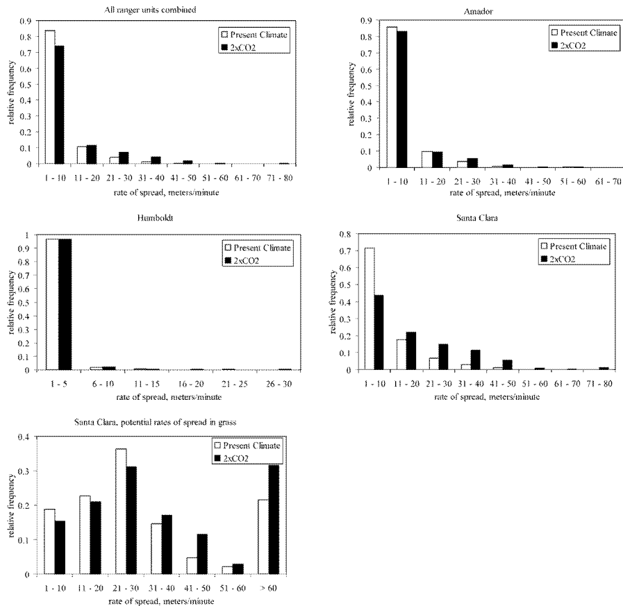
Figure 2. Frequency of predicted rates of spread (ROS) in m/min for 'historical' fires for Present Climate and 2 \times \text{CO}_2 climate change scenarios for (a) all three ranger units, (b) Amador ranger unit, (c) Humboldt ranger unit, (d) Santa Clara ranger unit, and (e) grass fuel Analysis Zones in the Santa Clara ranger unit.
