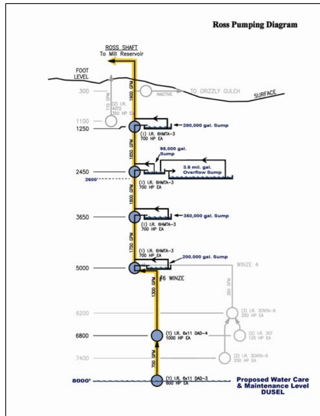
Ross Shaft Pumping Schematic
