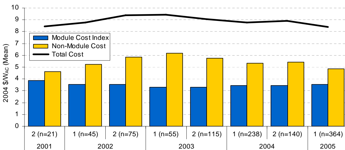
Figure 13. Installed Cost Over Time, by Module and Non-Module Costs (CPUC)
