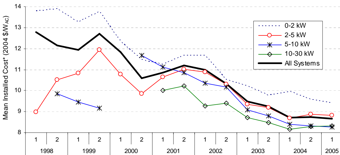
Figure 5. Average Installed Cost Over Time, by System Size (CEC)
