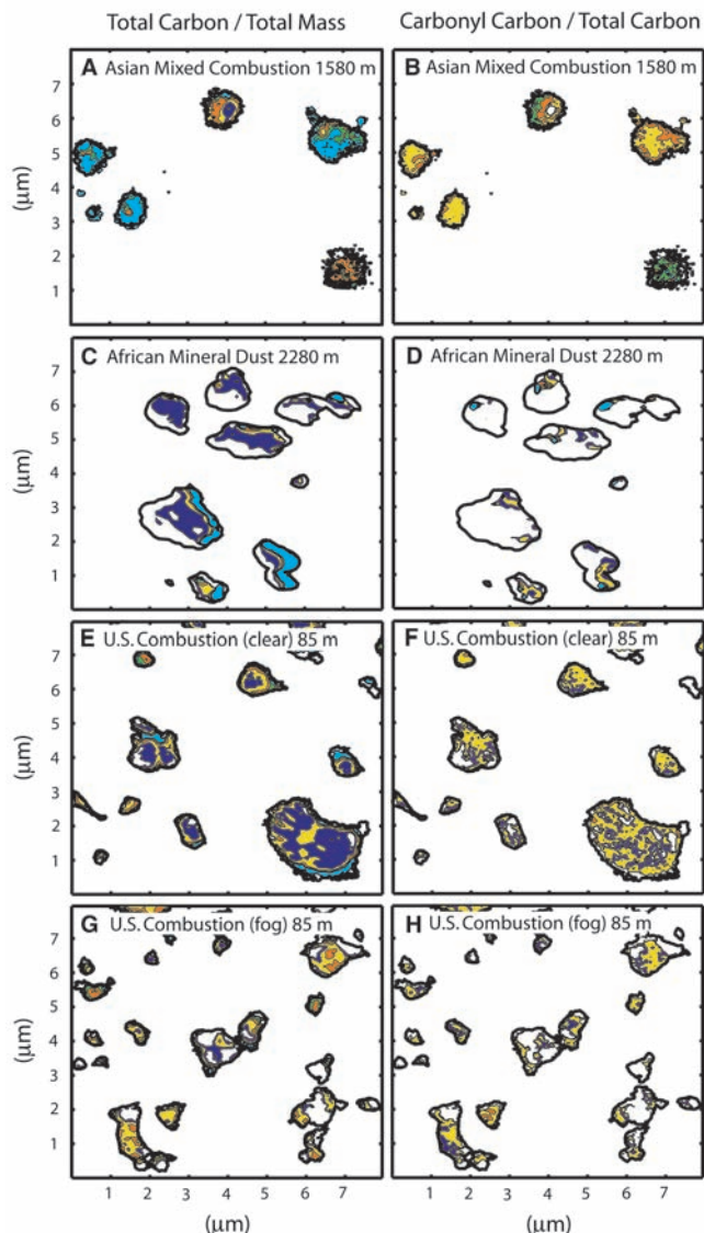
Fig. 4. Two-dimensional spectrally resolved maps of organic composition for particles representative of the four aerosol samples shown in Fig. 2. The total carbon-to-total mass ratios are plotted [(A), (C), (E), and (G)], demonstrating ratios of 0.02 to 0.2 (dark blue), 0.2 to 0.4 (yellow), 0.4 to 0.6 (orange), 0.6 to 0.8 (green), and >0.8 (light blue). The carbonyl-to-total carbon ratio is plotted [(B), (D), (F), and (H)], demonstrating ratios of 0.02 to 0.08 (dark blue), 0.08 to 0.16 (yellow), 0.16 to 0.24 (orange), 0.24 to 0.32 (green), and >0.32 (light blue). For chemically heterogeneous particles, regions of enhanced carbon and carbonyl concentrations can be identified as orange, green, or light blue areas in the plots shown here. The samples shown are [(A) and (B)] Asian combustion over the Sea of Japan on 27 April 2001, [(C) and (D)] African mineral dust over the Caribbean Sea on 21 July 2000, [(E) and (F)] eastern U.S. combustion in New Jersey on 12 August 2003, and [(G) and (H)] eastern U.S. combustion during fog in New Jersey on 7 August 2003. For all panels, black outlines indicate regions where the total mass is above the detection limit. The total mass detection limit and the particle edges are effectively coincident to within the precision of the STXM measurement. White regions indicate that total carbon or carbonyl carbon signatures are below detection.
