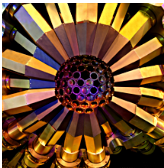
Figure 6-5. One hemisphere of the Gammasphere detector array.
